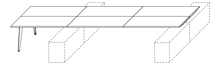
L. 4200/4800/5400 D/P. 1600
